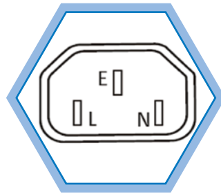
Socket Type: IEC 320 C13 Socket Parameter: Rating up to 10A
